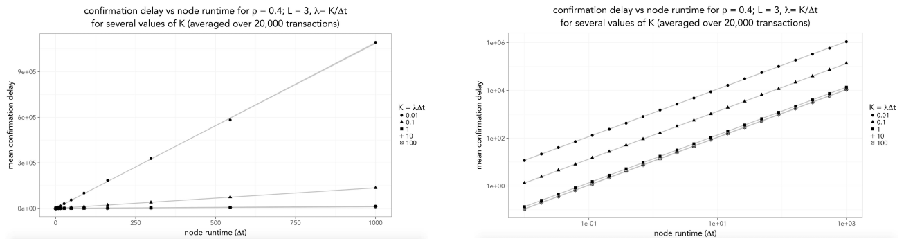
Figure 38: These figures show that the mean confirmation delay is significantly controlled by the parameter K . This means that as long as the rate of new transactions arriving is high enough, a complex proof-of-work is not detrimental to transaction throughput.
