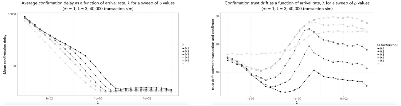
Figure 36: Note the inflection point slightly before \lambda = 10 . This appears to be universal and is likely related to the value of \lambda necessary to stop the DAG from becoming disconnected as is visible in Figure 31
