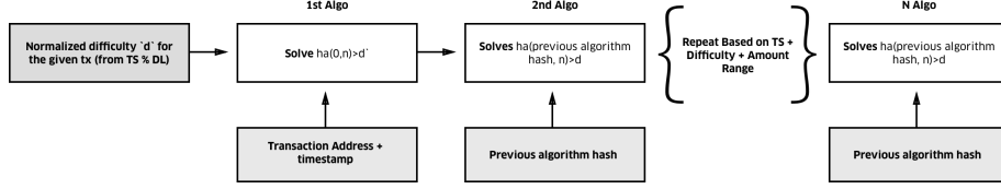
Figure 26: Proof of Work flow.
