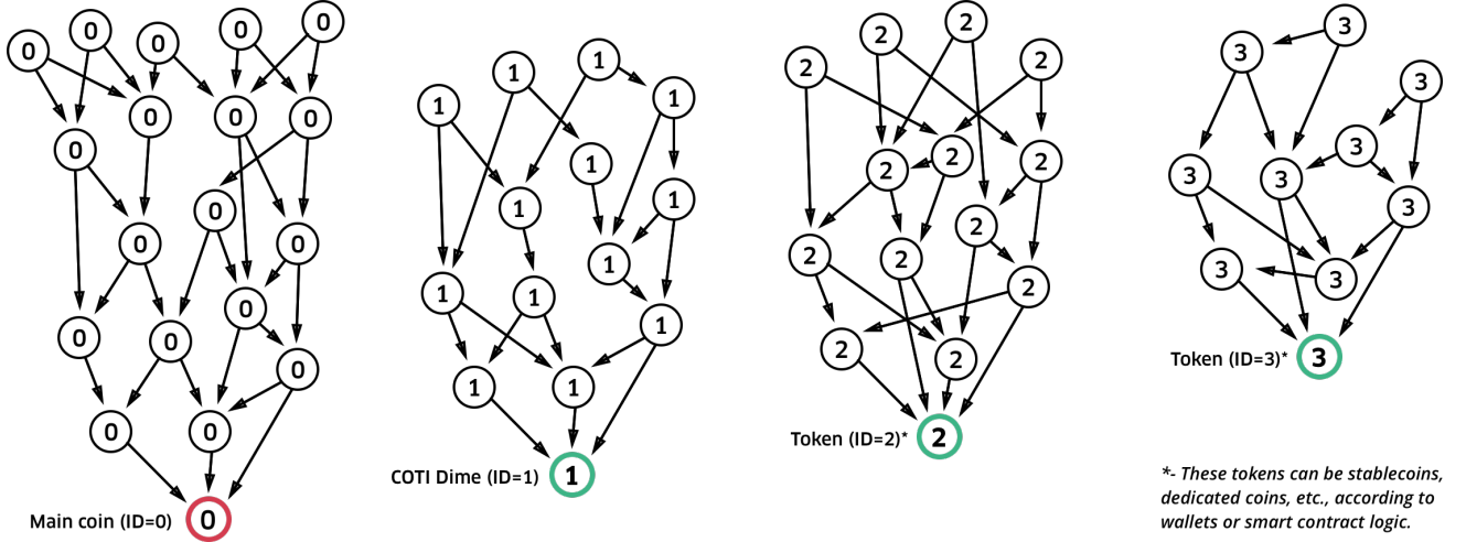
Figure 6: Multiple Clusters (DAGs) upon the same infrastructure
