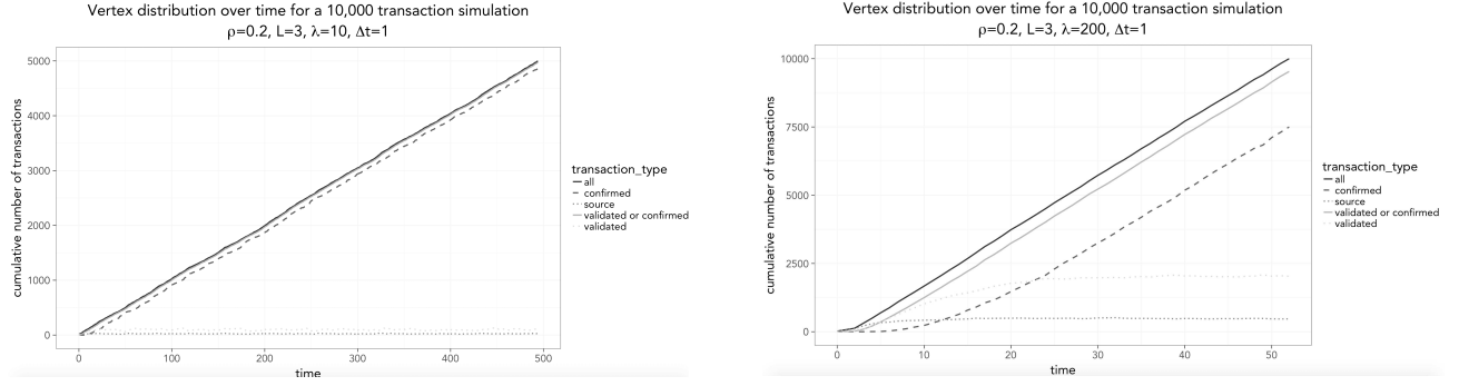
Figure 32: These figures show that after the initial phase, the system becomes stable and the rate at which transactions are confirmed equals the rate at which new transactions arrive. In particular, the number of sources and number of new (not yet validated) transactions becomes constant.
