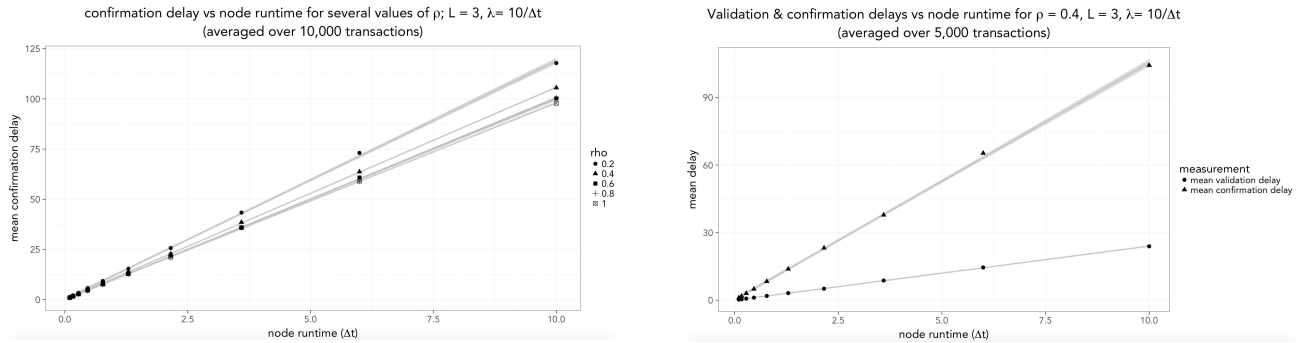
Figure 37: The figure on the left shows the confirmation time is barely affected by the size of the threshold \rho . The figure on the right shows that the mean delay in validation and confirmation times are directly proportional to the time taken to run the Source Selection Algorithm and to do the proof-of-work ( \Delta t ).
