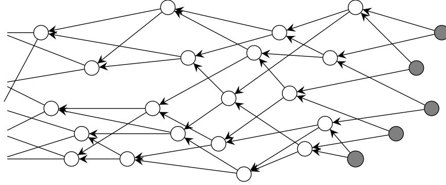
Figure 30: The Clusterstamp process captures all the information up to the time of the gray transactions. Thereafter, the next generation of the Cluster begins with the gray transactions.
