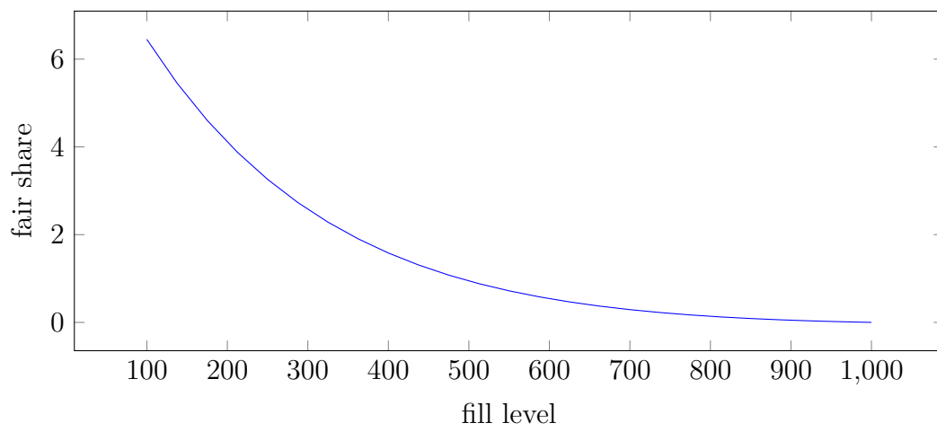
Figure 3: fair share for effective importance of 1‰
