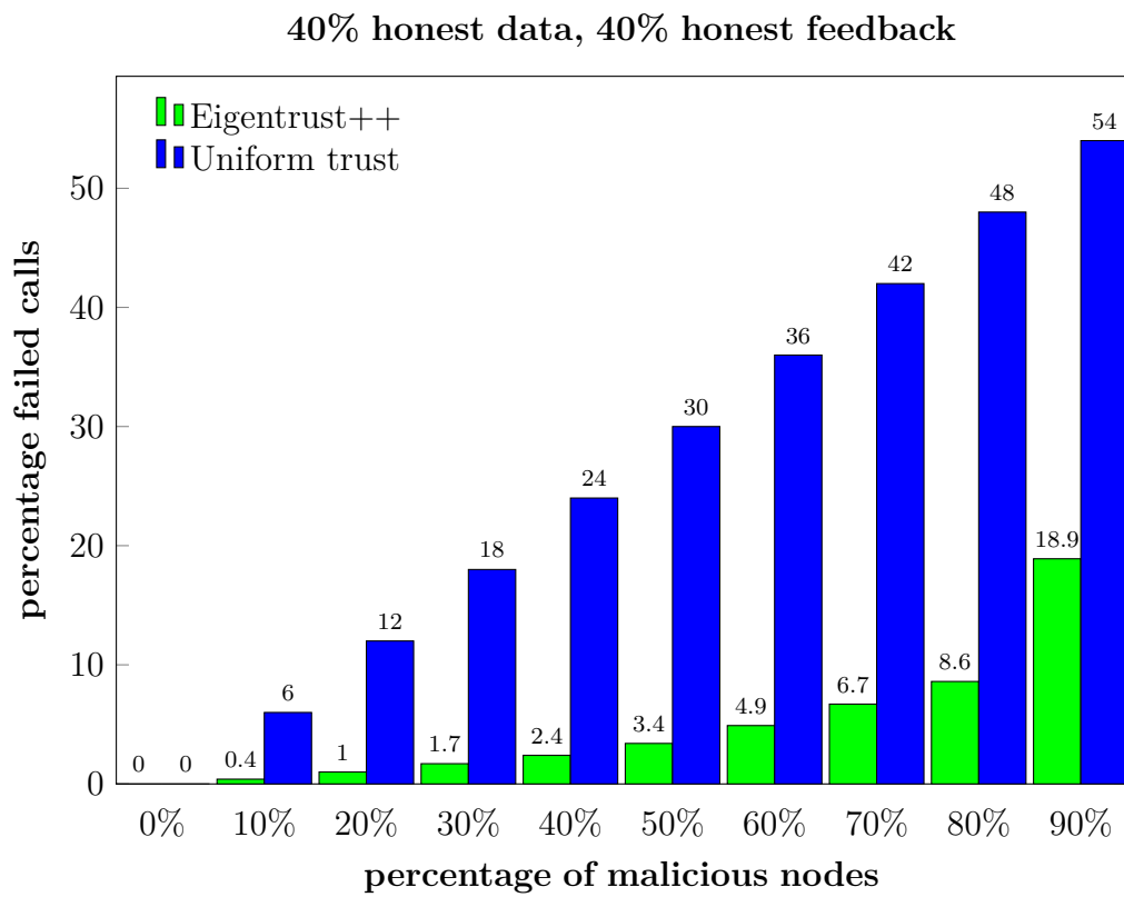
Figure 7: Simulation with attacking nodes that are sometimes dishonest
