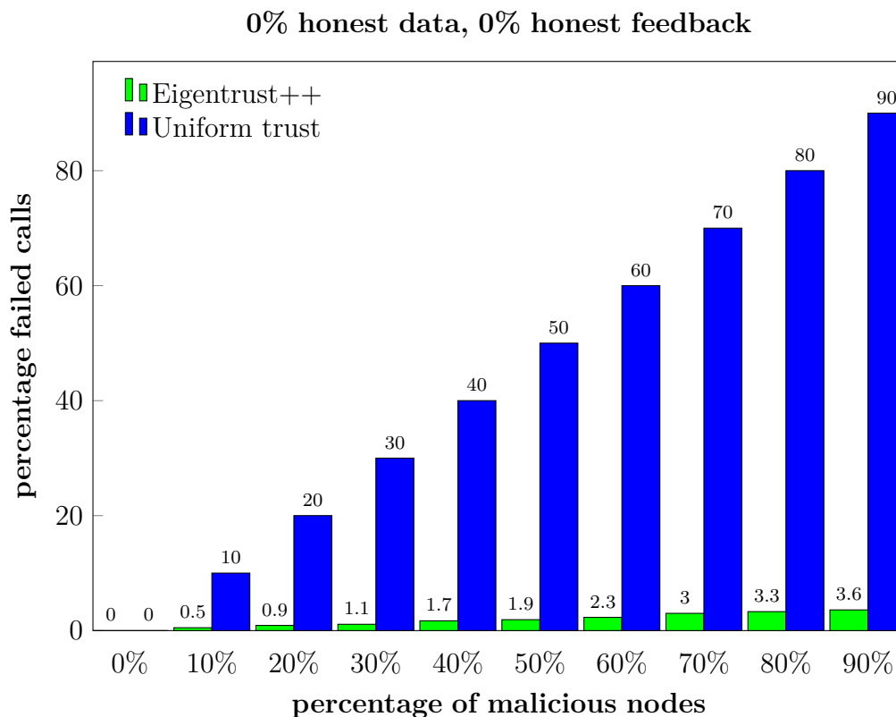
Figure 6: Simulation with attacking nodes that are always dishonest
