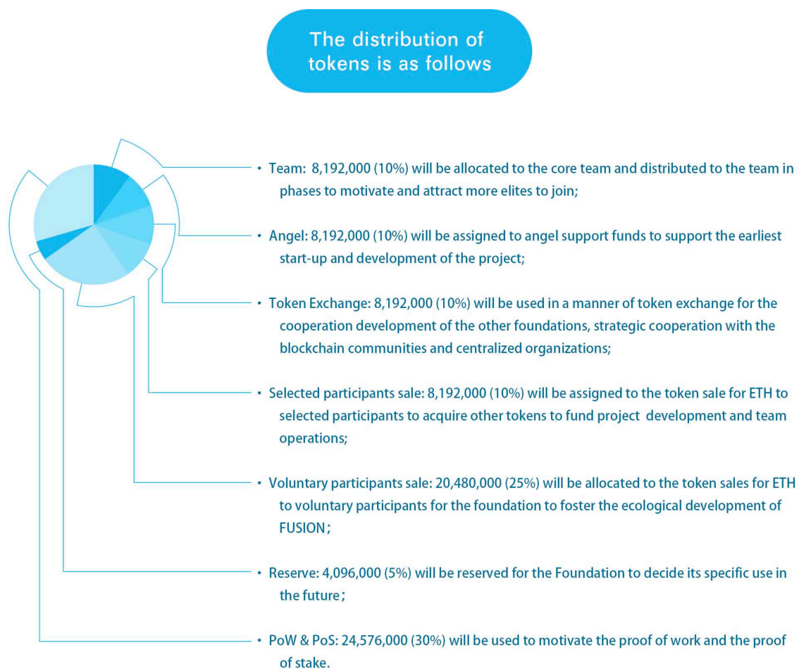
Figure 17. Token distribution
